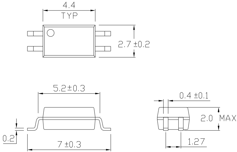
Package Drawing (Dimensions in mm)
