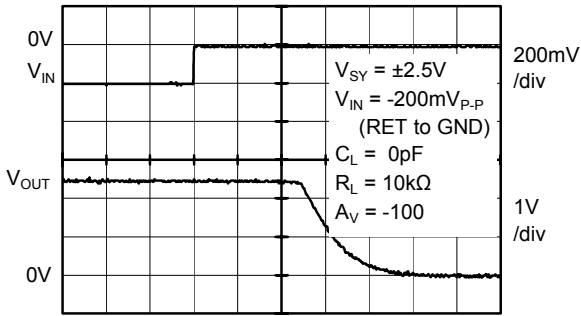
Time (20µs/div)
