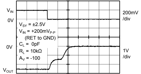
Time (50µs/div)
