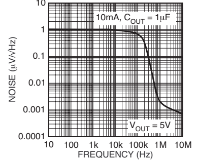
Noise Performance
