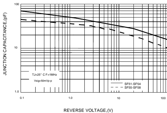
FIG.5-TYPICAL JUNCTION CAPACITANCE
