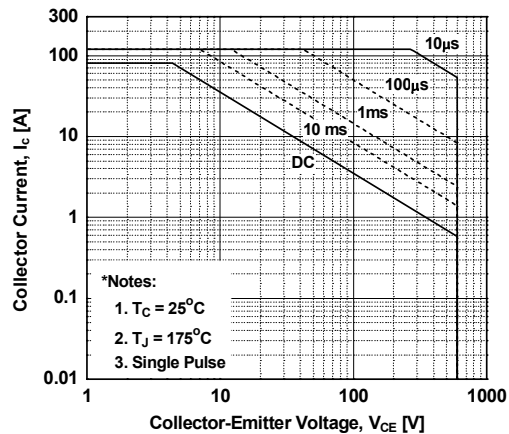
Figure 11. SOA Characteristics
