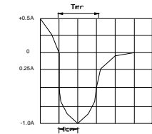
FIG.6-TEST CIRCUIT DIAGRAM AND REVERSE RECOVERY TIME CHARACTERISTIC
